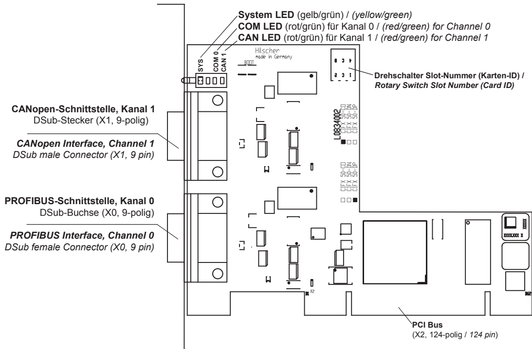
Figure 10: CIFX 50-2DP\CO (Hardware Revision 2)
