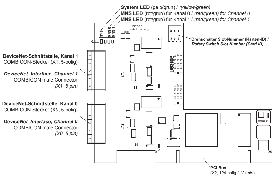
Figure 24: CIFX 50-2DN (Hardware Revision 2)
