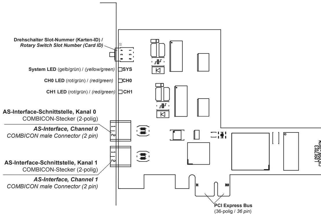
Figure 27: CIFX 50E-2ASM (from hardware revision 2)
