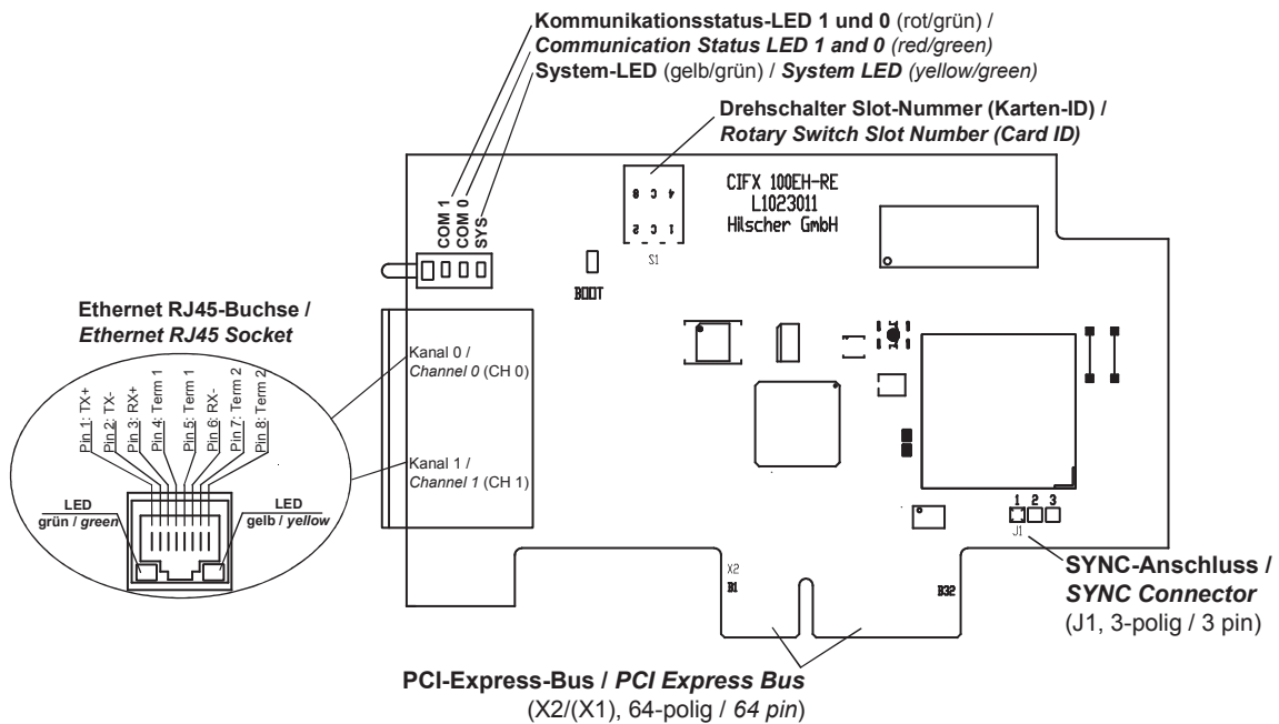
Figure 35: CIFX 100EH-RE\CUBE*
