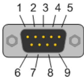
Figure 51: CANopen Interface (DSub male connector, 9 pin), X400
