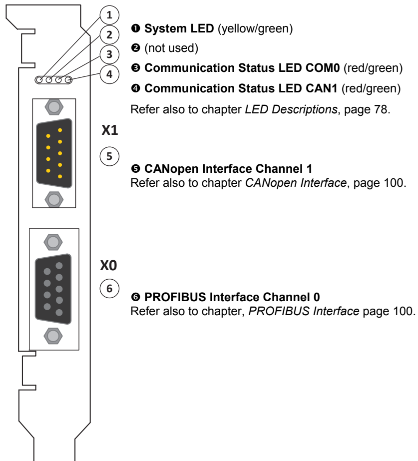
Figure 11: Front Plate CIFX 50-2DP\CO
