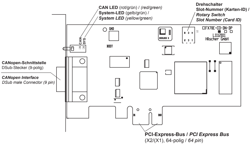
Figure 41: CIFX 70E-CO\MR (Hardware revision 1)
