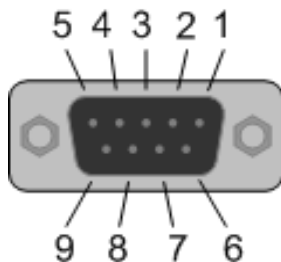
Figure 50: PROFIBUS Interface (DSub female connector, 9 pin), X400
