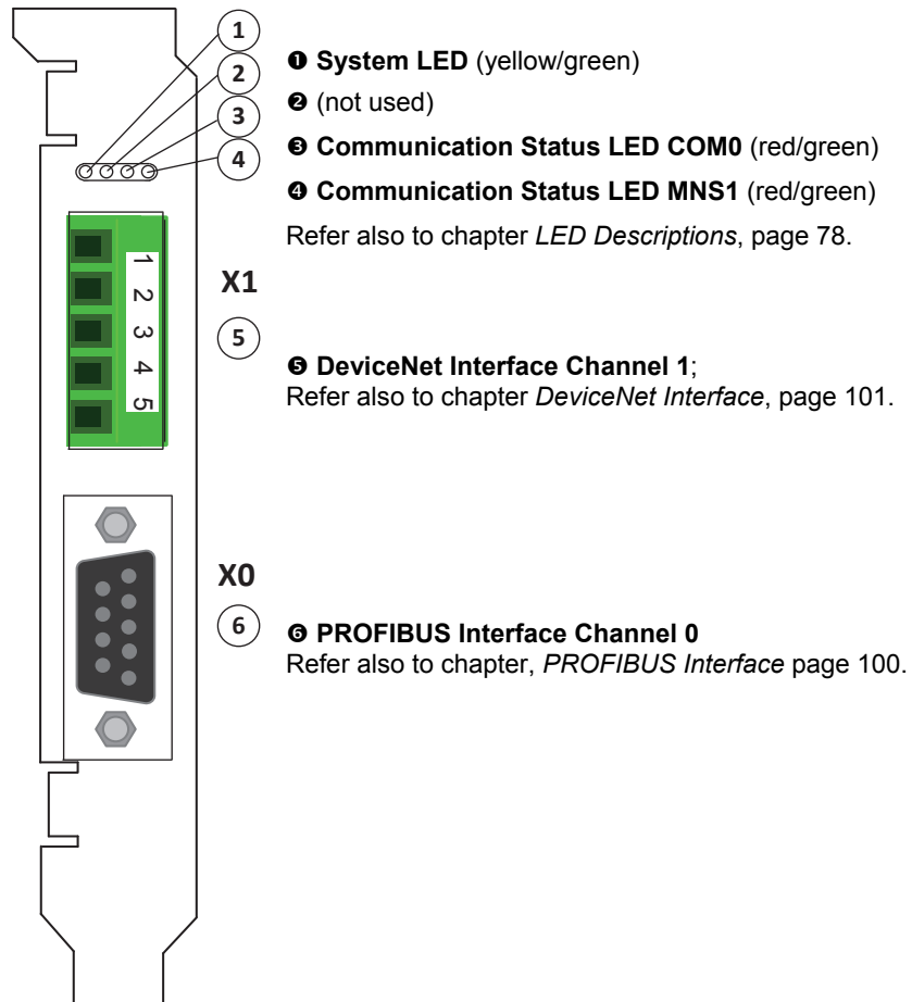
Figure 13: Front Plate CIFX 50-2DP\DN
