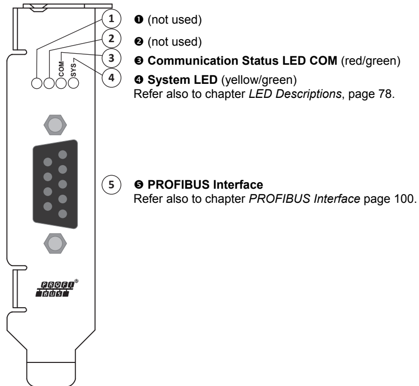
Figure 39: Front Plate CIFX 70E-DP, CIFX 70E-DP1MR
