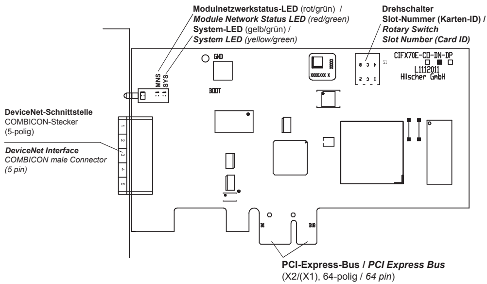
Figure 43: CIFX 70E-DN (Hardware revision 1)
