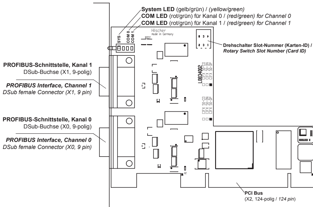
Figure 8: CIFX 50-2DP (Hardware Revision 3)
